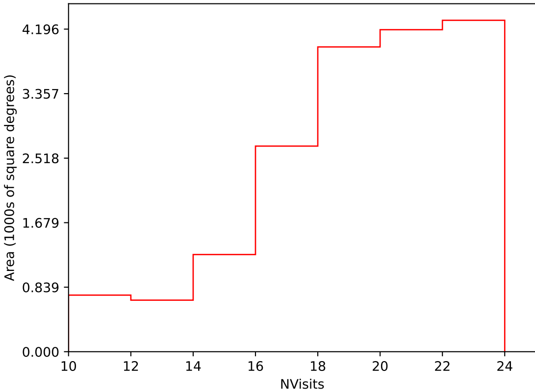
too_elab_heavy_r128_d3_gz_v3.4_10yrs Yr 1 i band: NVisits
