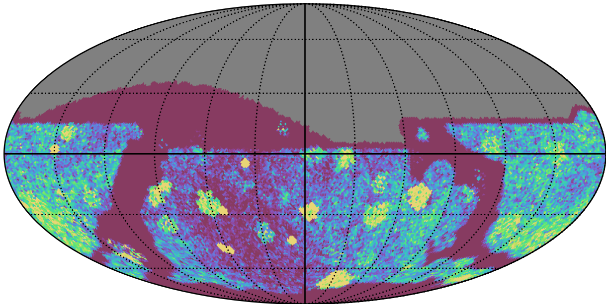
too_elab_heavy_r128_d3_gz_v3.4_10yrs Yr 1 all bands: NVisits
