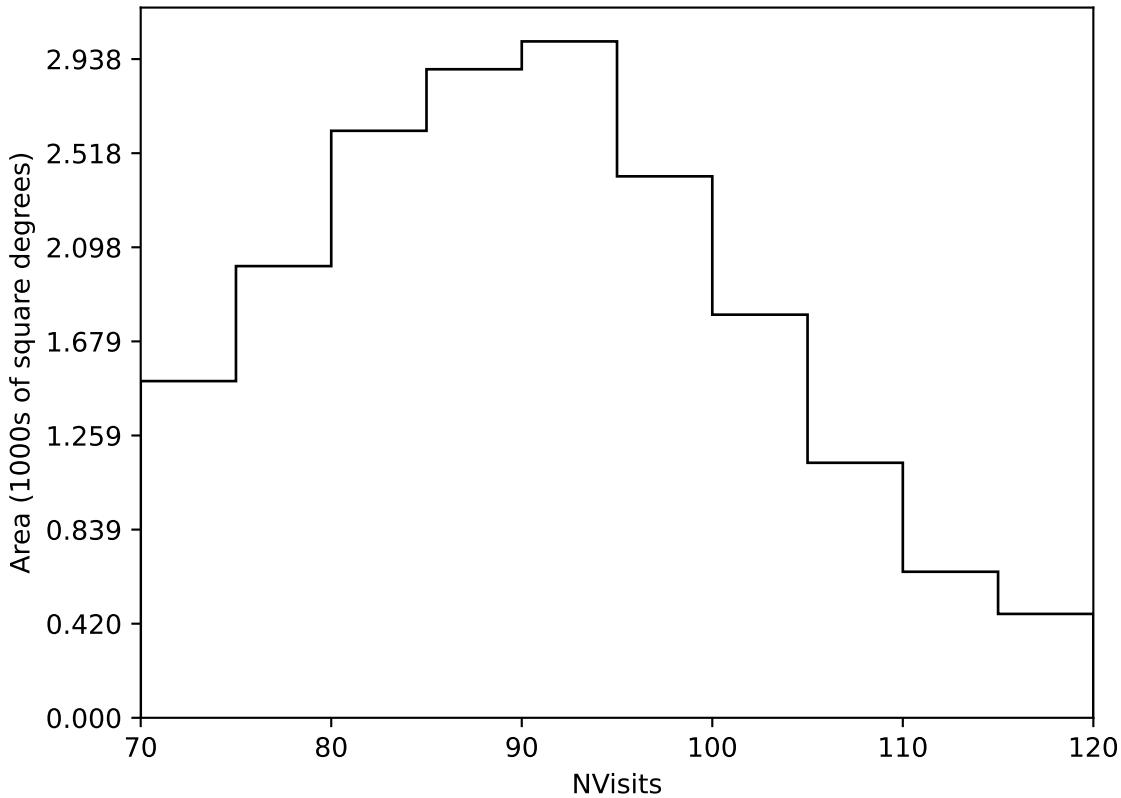
too_elab_heavy_r128_d3_gz_v3.4_10yrs Yr 1 all bands: NVisits
