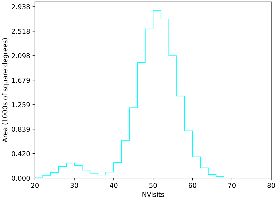
too_elab_heavy_r128_d3_gz_v3.4_10yrs WFD u band: NVisits
