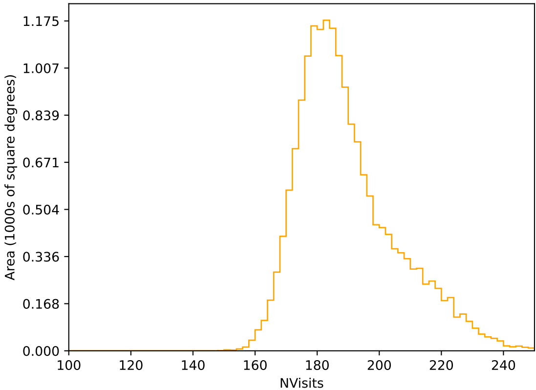
too_elab_heavy_r128_d3_gz_v3.4_10yrs WFD r band: NVisits
