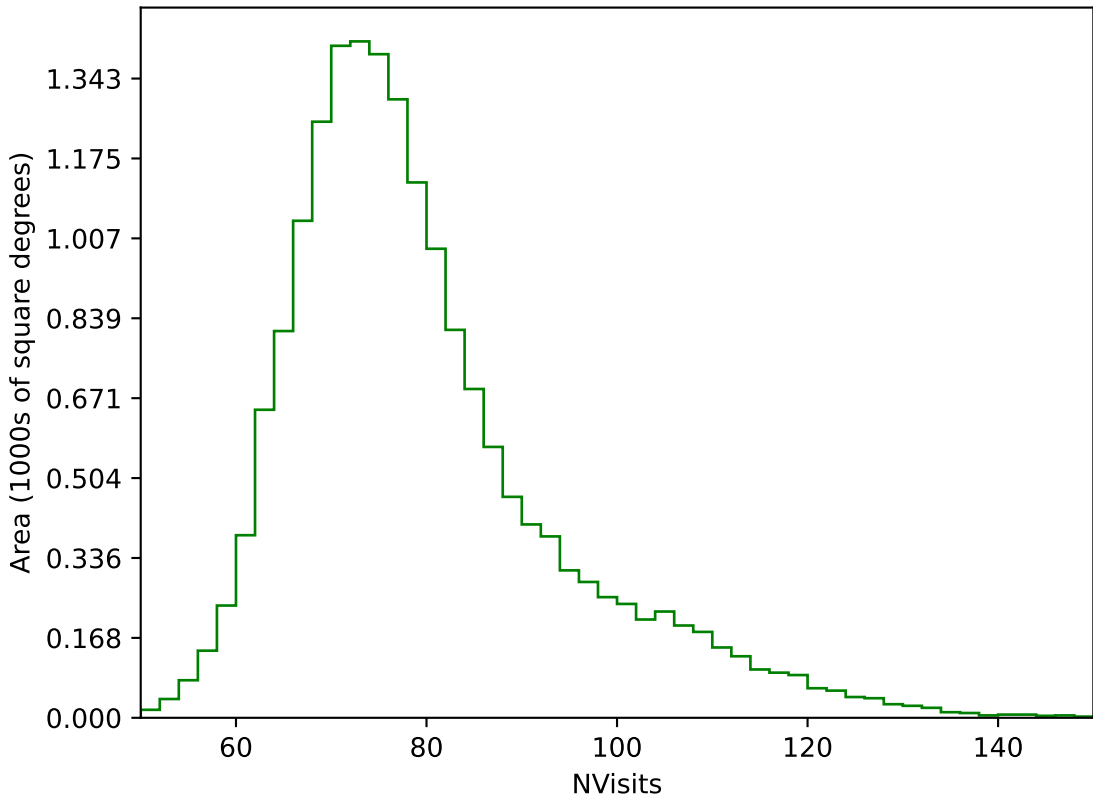
too_elab_heavy_r128_d3_gz_v3.4_10yrs WFD g band: NVisits
