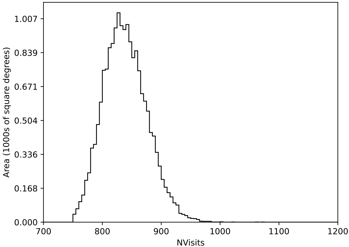
too_elab_heavy_r128_d3_gz_v3.4_10yrs WFD all bands: NVisits
