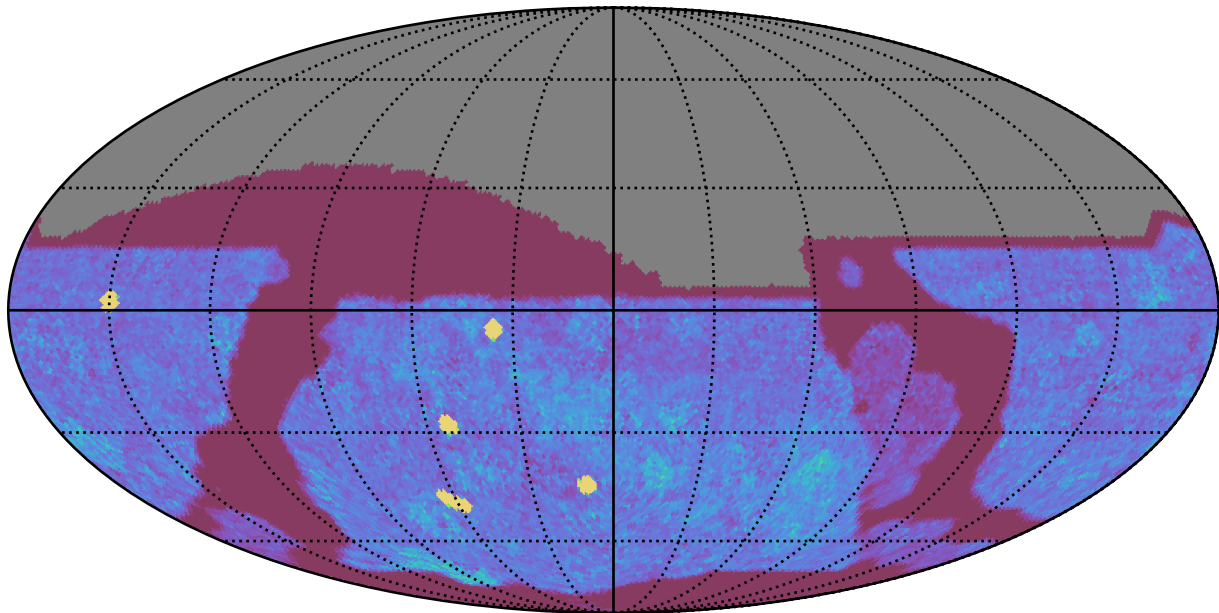
too_elab_heavy_r128_d3_gz_v3.4_10yrs All sky z band: NVisits
