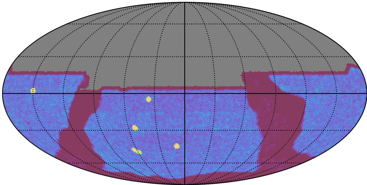
too_elab_heavy_r128_d3_gz_v3.4_10yrs All sky y band: NVisits
