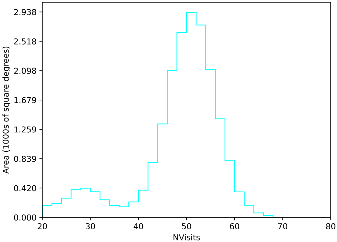
too_elab_heavy_r128_d3_gz_v3.4_10yrs All sky u band: NVisits
