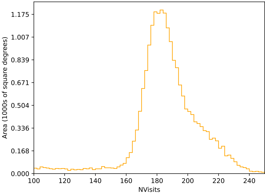
too_elab_heavy_r128_d3_gz_v3.4_10yrs All sky r band: NVisits
