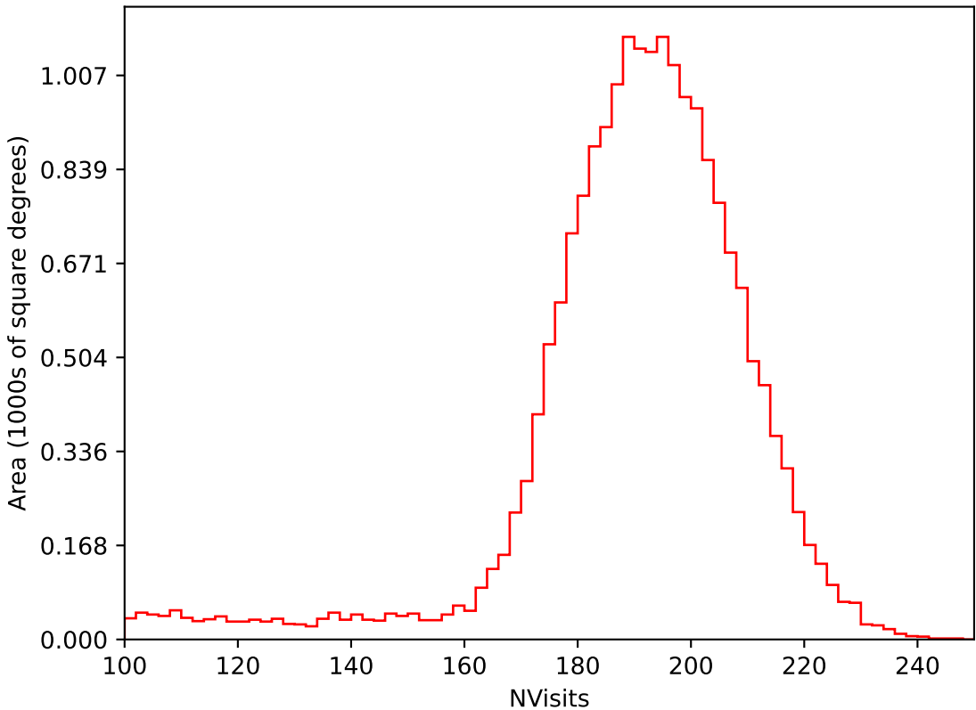
too_elab_heavy_r128_d3_gz_v3.4_10yrs All sky i band: NVisits
