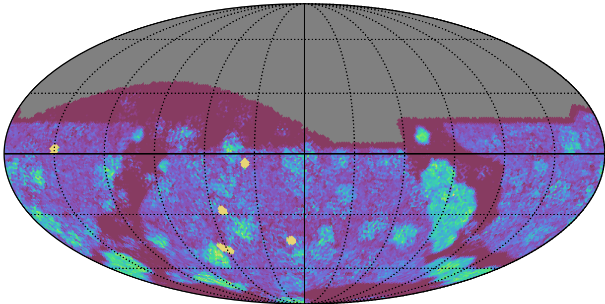
too_elab_heavy_r128_d3_gz_v3.4_10yrs All sky g band: NVisits
