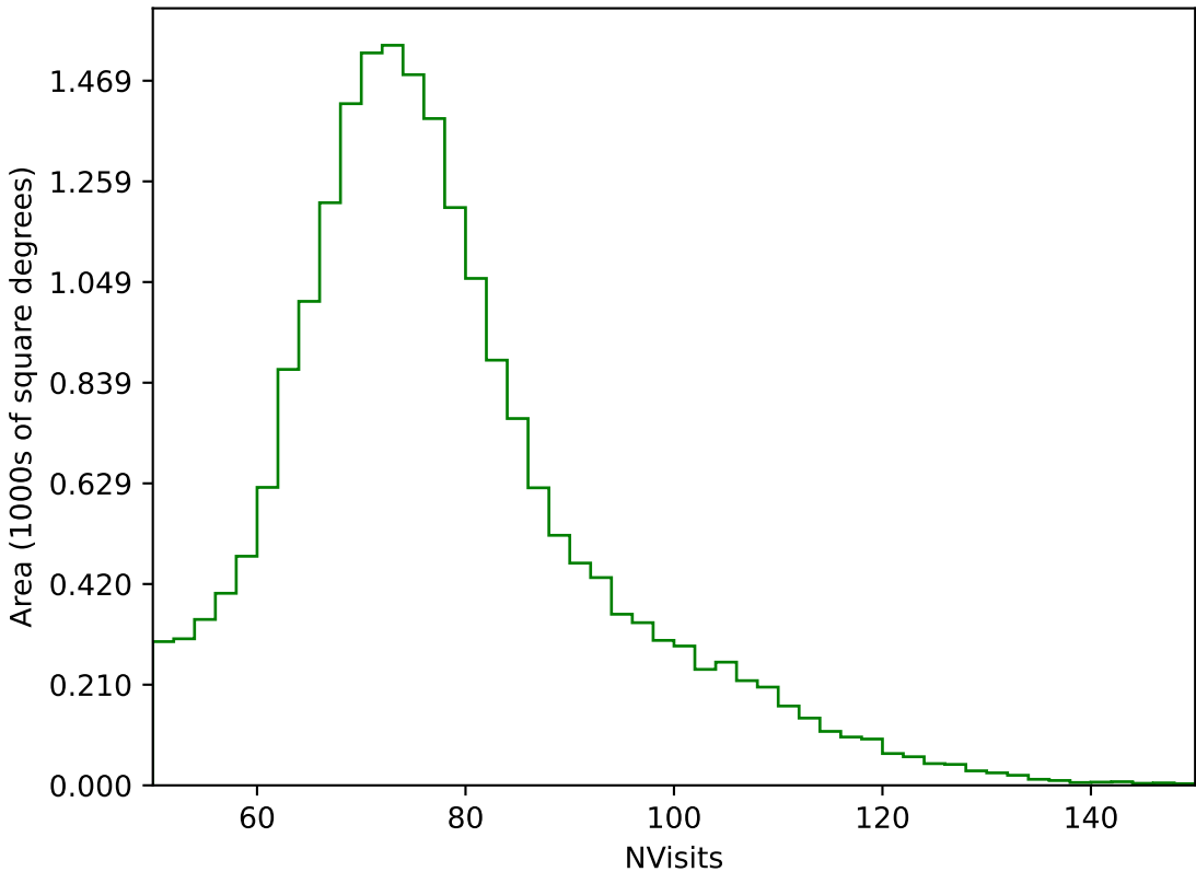
too_elab_heavy_r128_d3_gz_v3.4_10yrs All sky g band: NVisits
