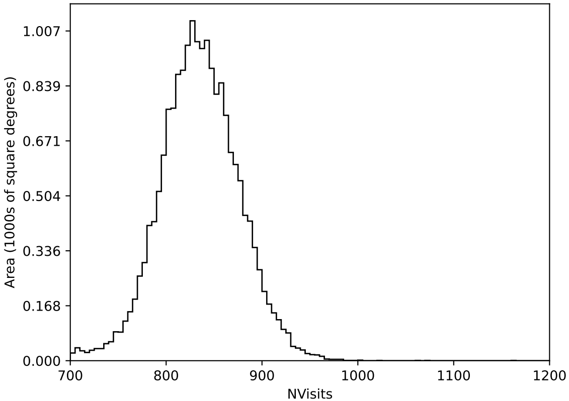
too_elab_heavy_r128_d3_gz_v3.4_10yrs All sky all bands: NVisits
