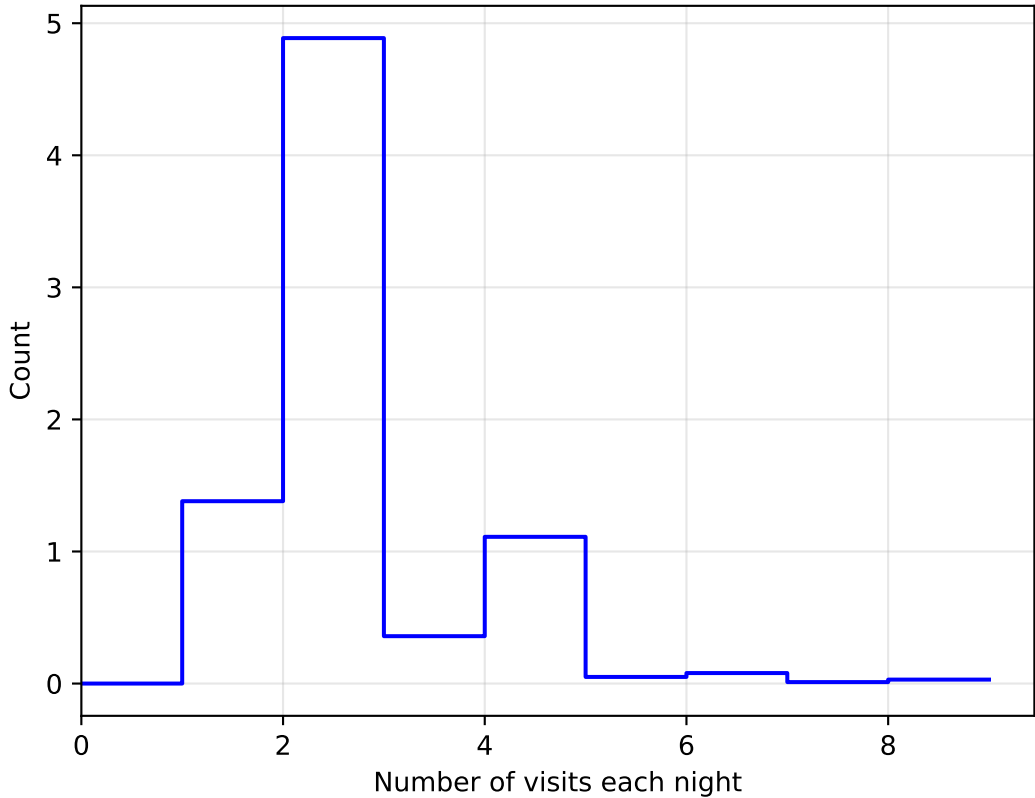
too_elab_heavy_r128_d3_gz_v3.4_10yrs WFD: NVisitsPerNight 1e6
