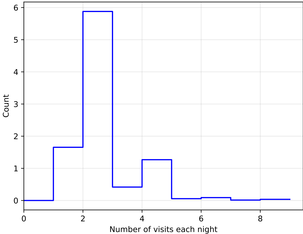
too_elab_heavy_r128_d3_gz_v3.4_10yrs All sky: NVisitsPerNight 1e6
