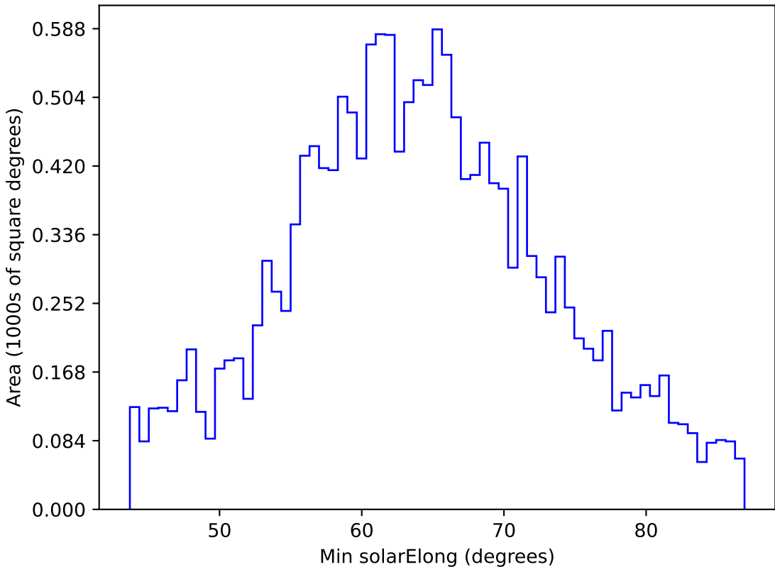
too_elab_heavy_r128_d3_gz_v3.4_10yrs WFD y band: Min solarElong
