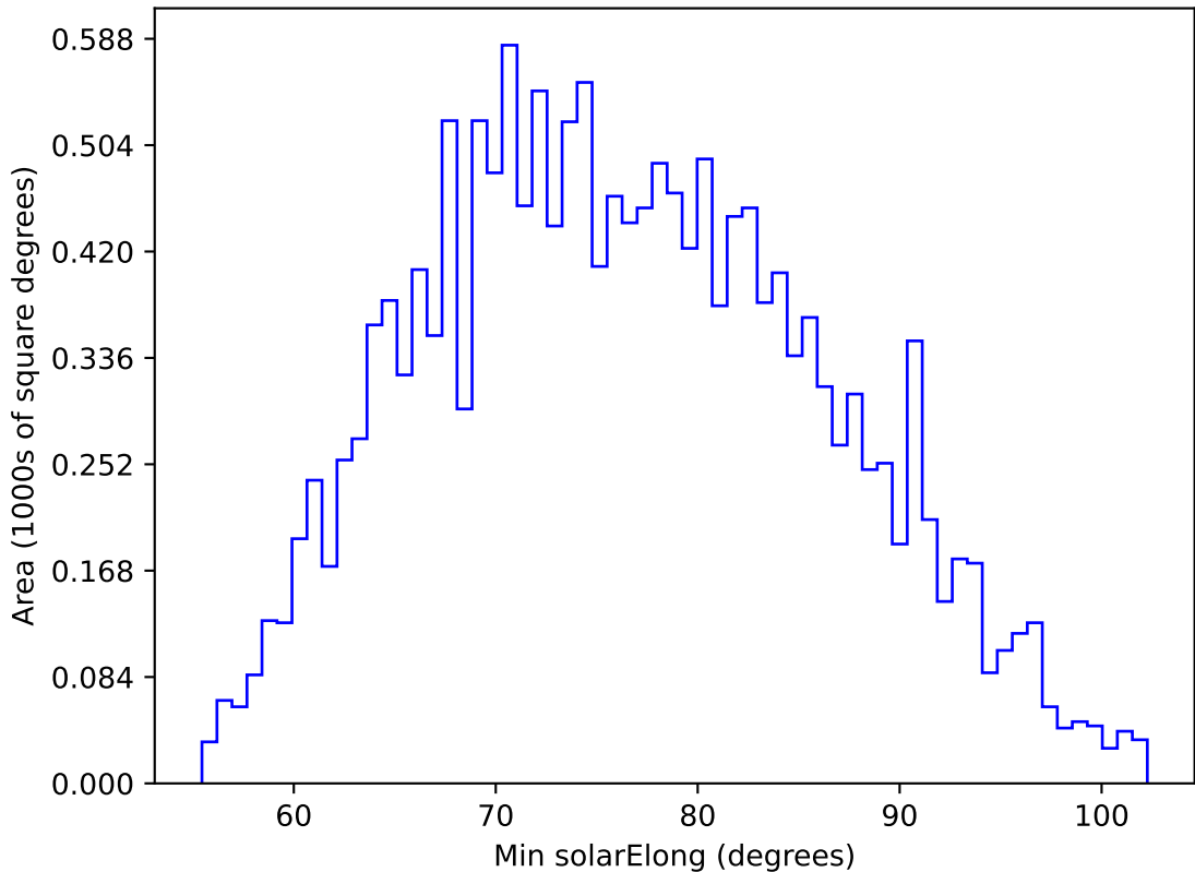
too_elab_heavy_r128_d3_gz_v3.4_10yrs WFD u band: Min solarElong
