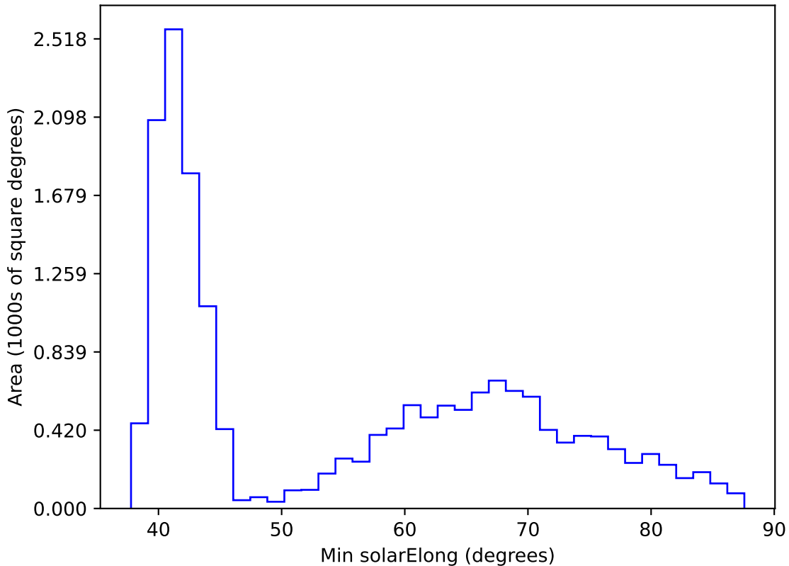
too_elab_heavy_r128_d3_gz_v3.4_10yrs WFD r band: Min solarElong
