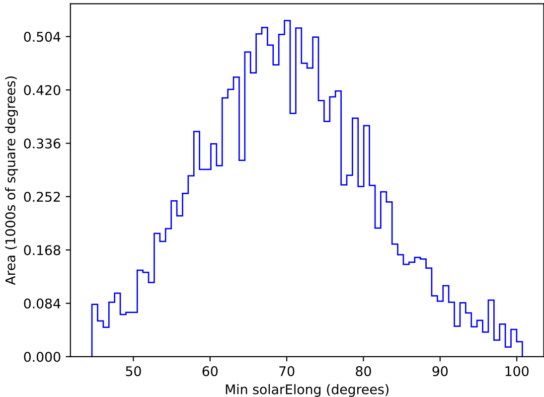
too_elab_heavy_r128_d3_gz_v3.4_10yrs WFD g band: Min solarElong
