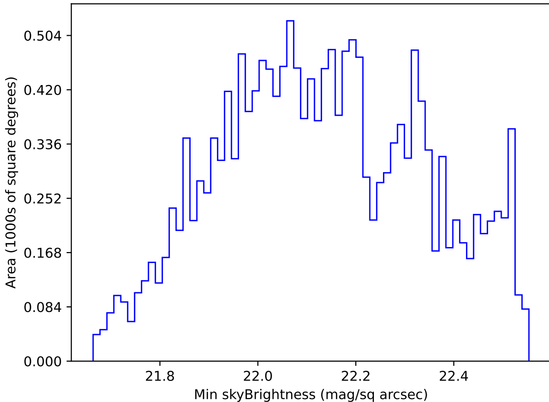
too_elab_heavy_r128_d3_gz_v3.4_10yrs WFD u band: Min skyBrightness
