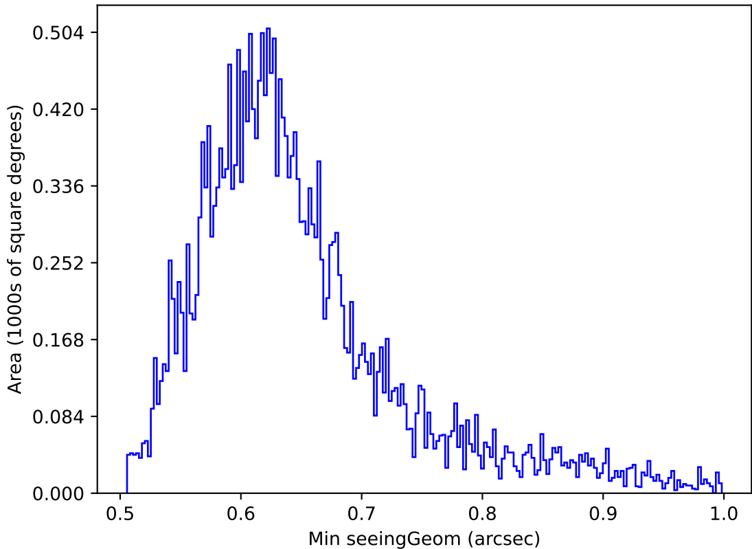
too_elab_heavy_r128_d3_gz_v3.4_10yrs Yr 1 z band: Min seeingGeom
