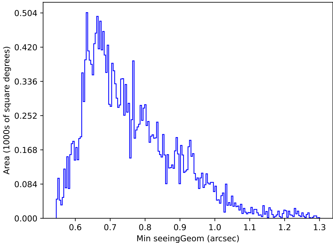
too_elab_heavy_r128_d3_gz_v3.4_10yrs Yr 1 u band: Min seeingGeom
