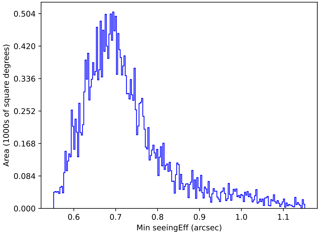
too_elab_heavy_r128_d3_gz_v3.4_10yrs Yr 1 z band: Min seeingEff
