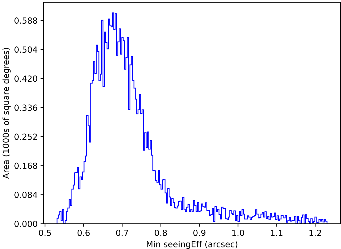
too_elab_heavy_r128_d3_gz_v3.4_10yrs Yr 1 r band: Min seeingEff
