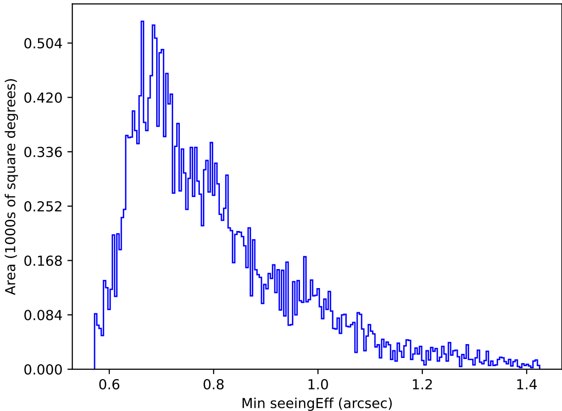
too_elab_heavy_r128_d3_gz_v3.4_10yrs Yr 1 g band: Min seeingEff
