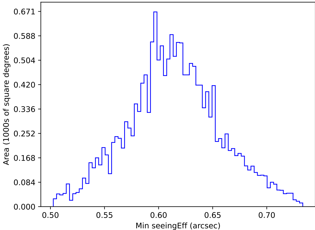
too_elab_heavy_r128_d3_gz_v3.4_10yrs WFD z band: Min seeingEff
