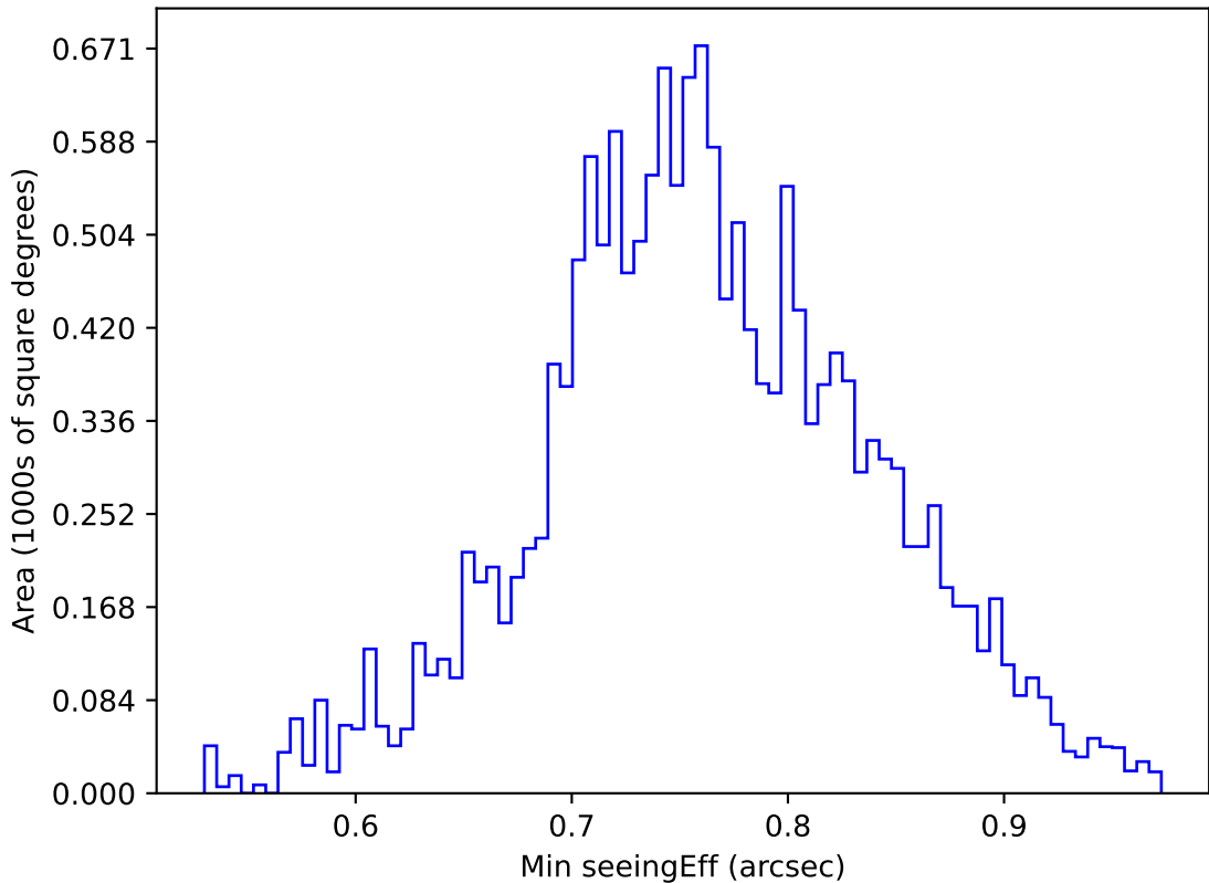
too_elab_heavy_r128_d3_gz_v3.4_10yrs WFD u band: Min seeingEff
