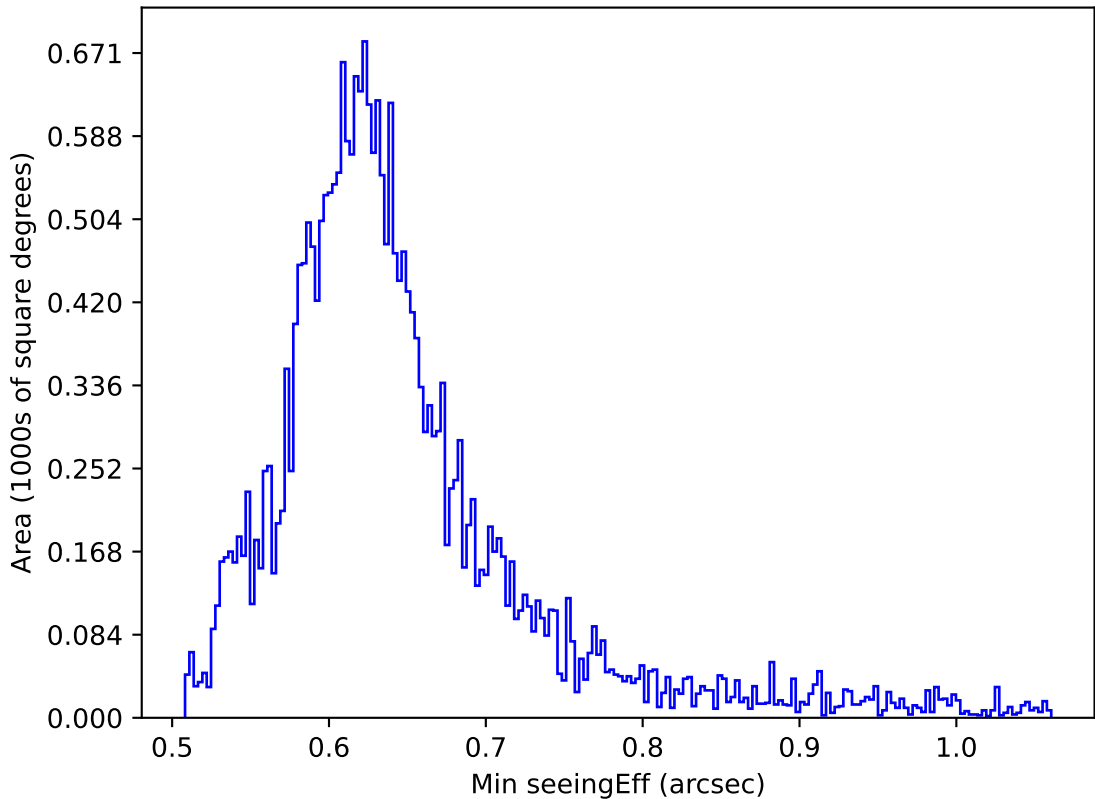
too_elab_heavy_r128_d3_gz_v3.4_10yrs All sky r band: Min seeingEff
