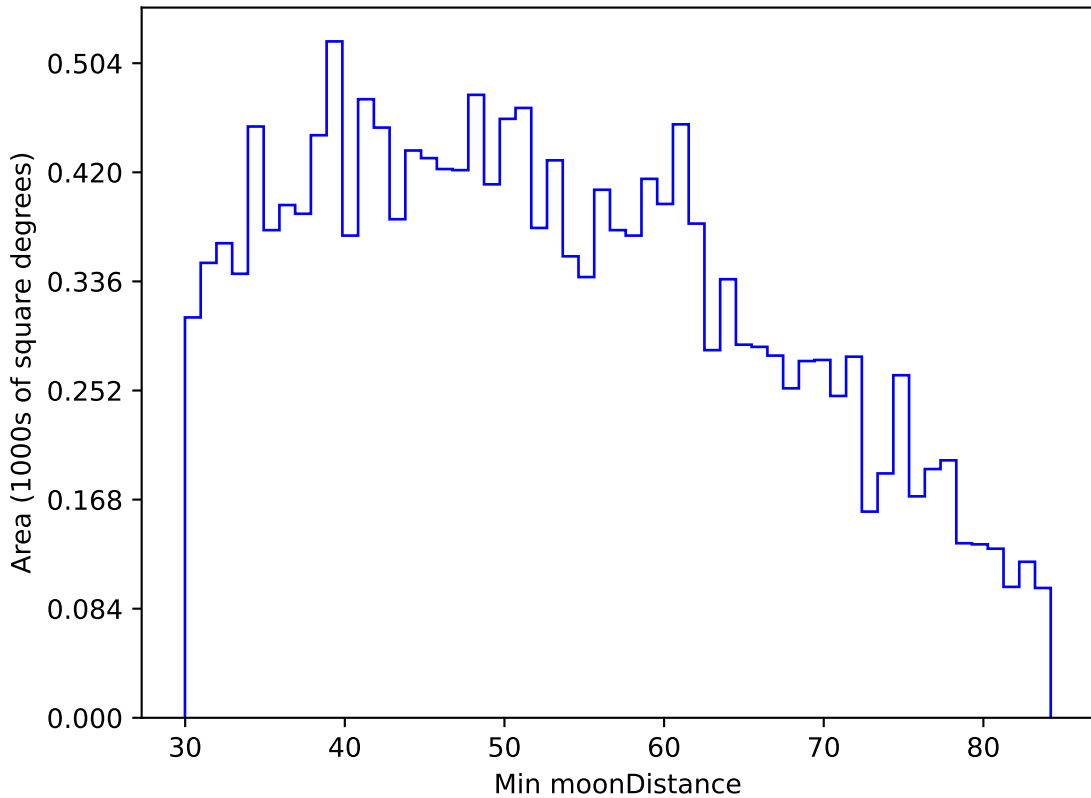
too_elab_heavy_r128_d3_gz_v3.4_10yrs WFD u band: Min moonDistance
