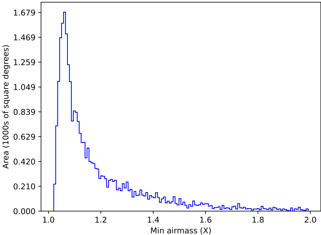
too_elab_heavy_r128_d3_gz_v3.4_10yrs Yr 1 g band: Min airmass
