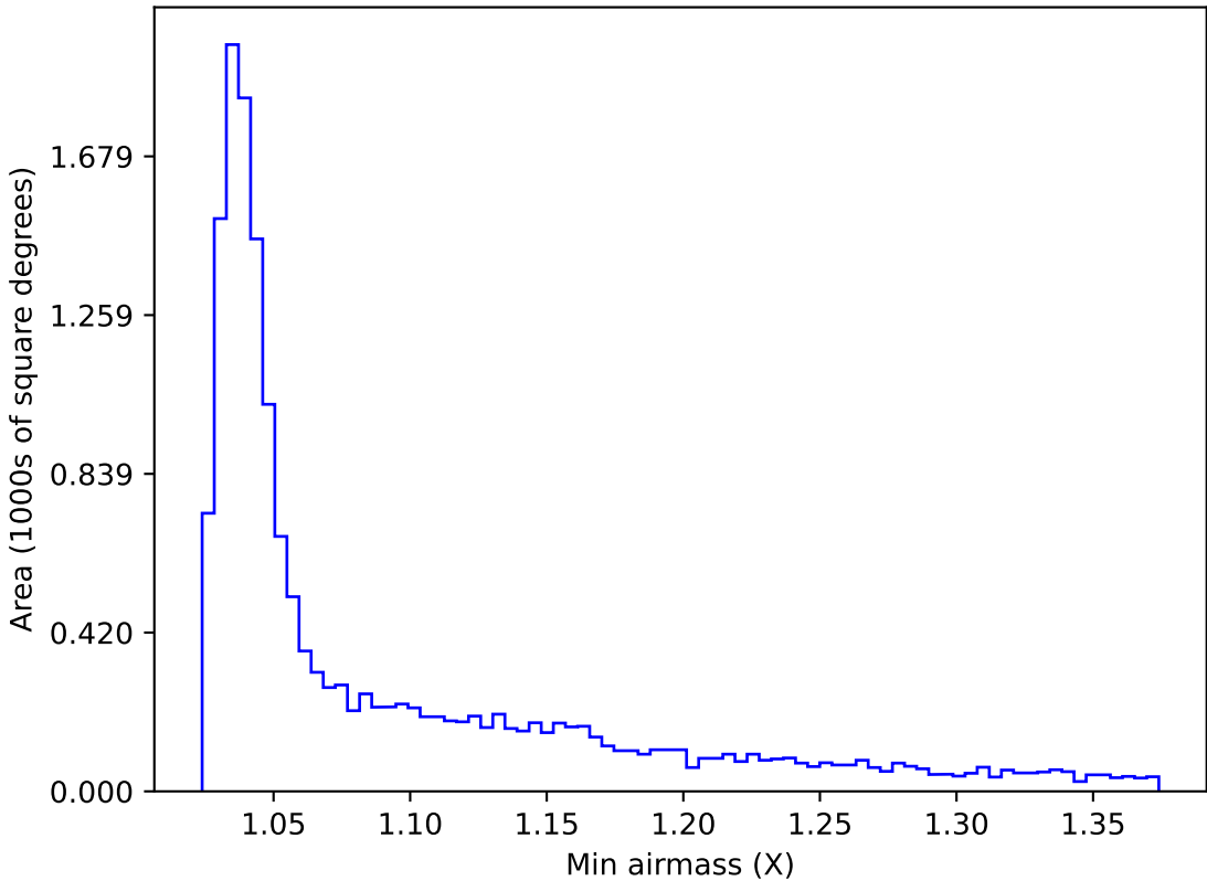
too_elab_heavy_r128_d3_gz_v3.4_10yrs WFD u band: Min airmass
