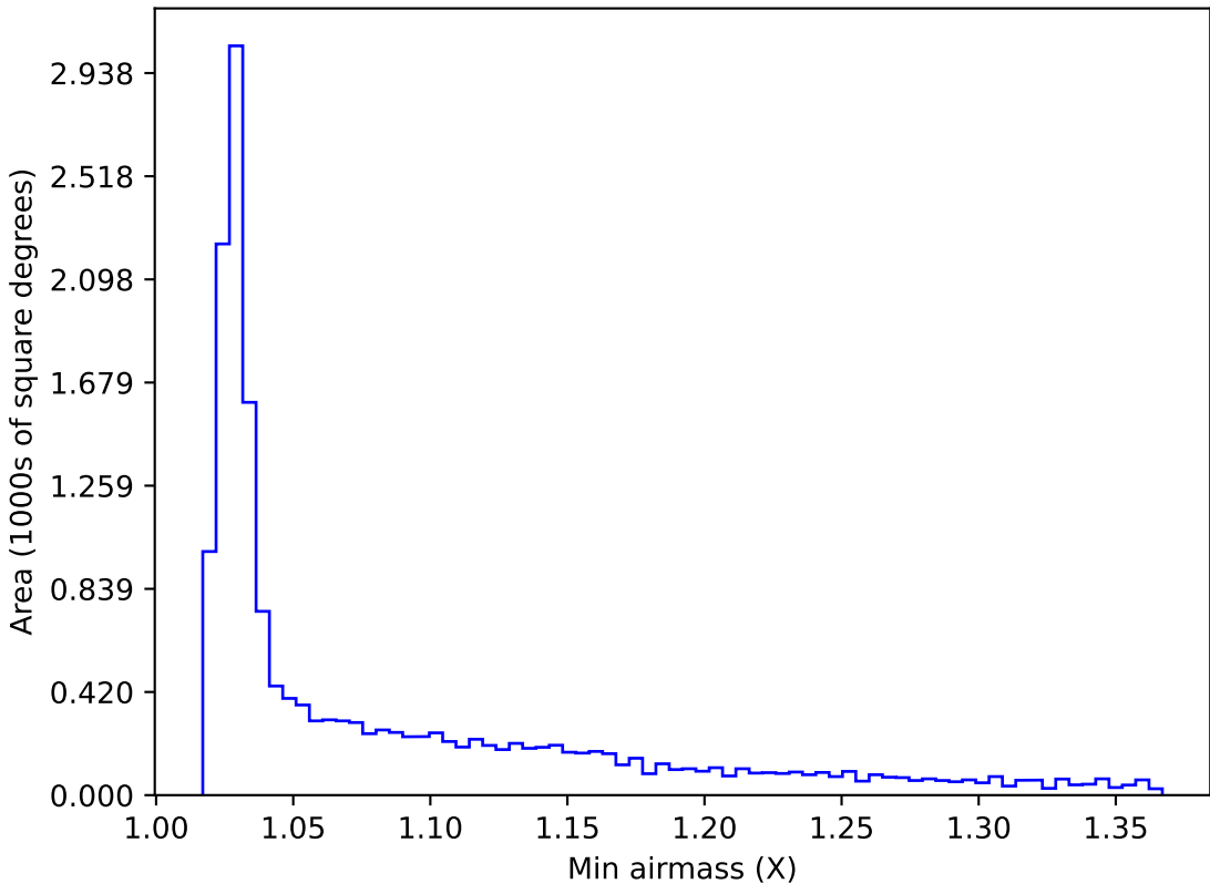
too_elab_heavy_r128_d3_gz_v3.4_10yrs WFD r band: Min airmass
