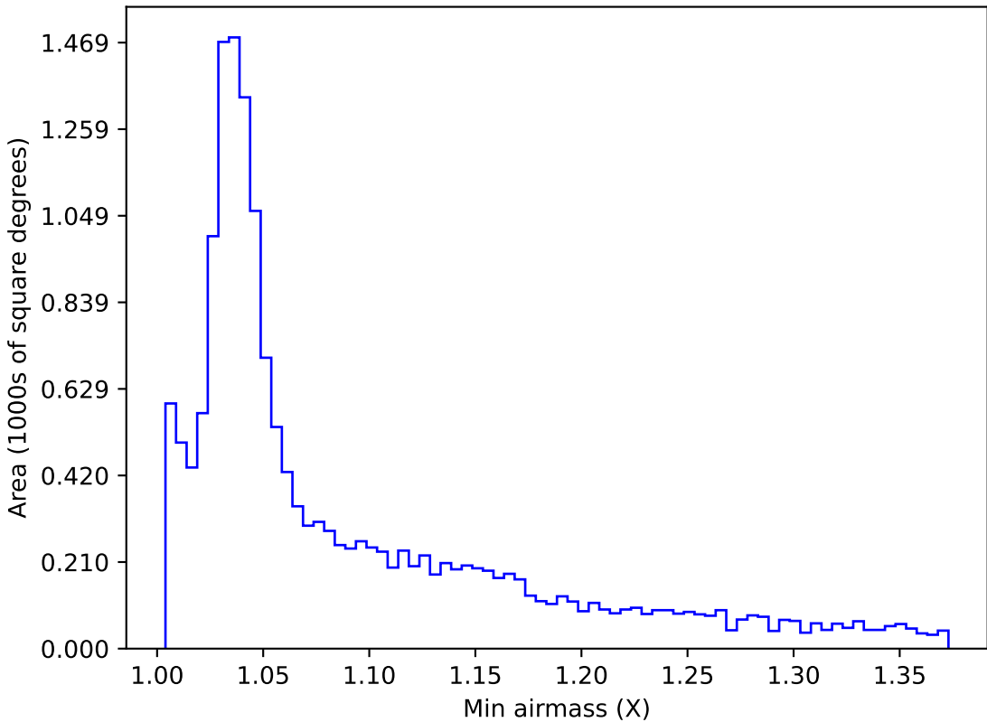
too_elab_heavy_r128_d3_gz_v3.4_10yrs WFD g band: Min airmass
