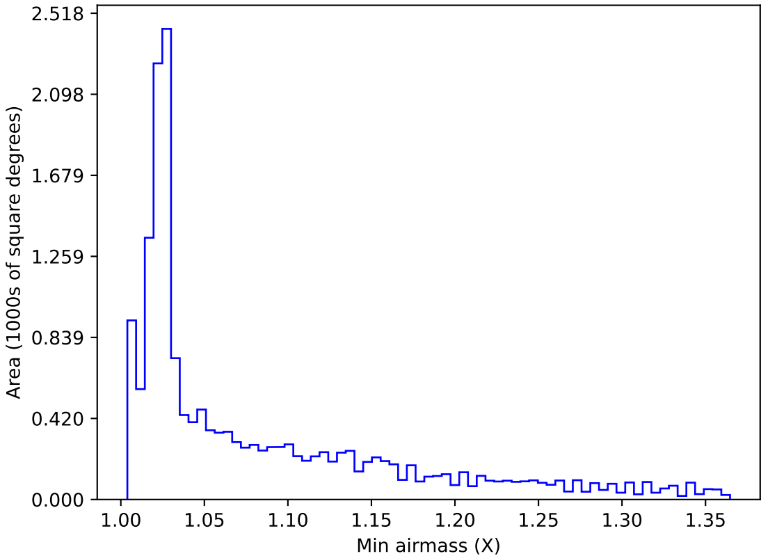
too_elab_heavy_r128_d3_gz_v3.4_10yrs WFD all bands: Min airmass
