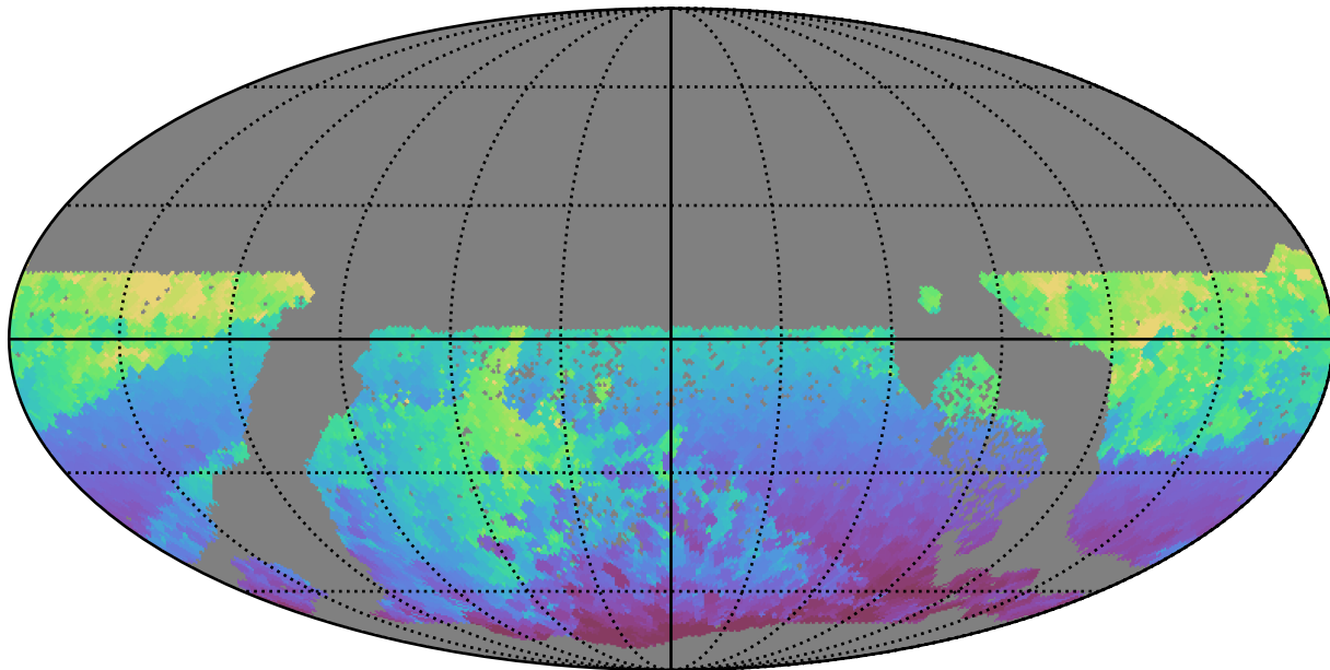
too_elab_heavy_r128_d3_gz_v3.4_10yrs WFD r band: Min HA
