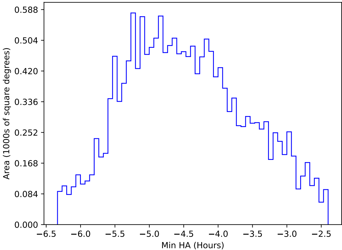
too_elab_heavy_r128_d3_gz_v3.4_10yrs WFD r band: Min HA
