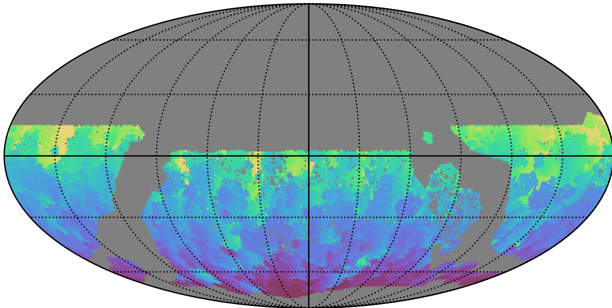
too_elab_heavy_r128_d3_gz_v3.4_10yrs WFD g band: Min HA
