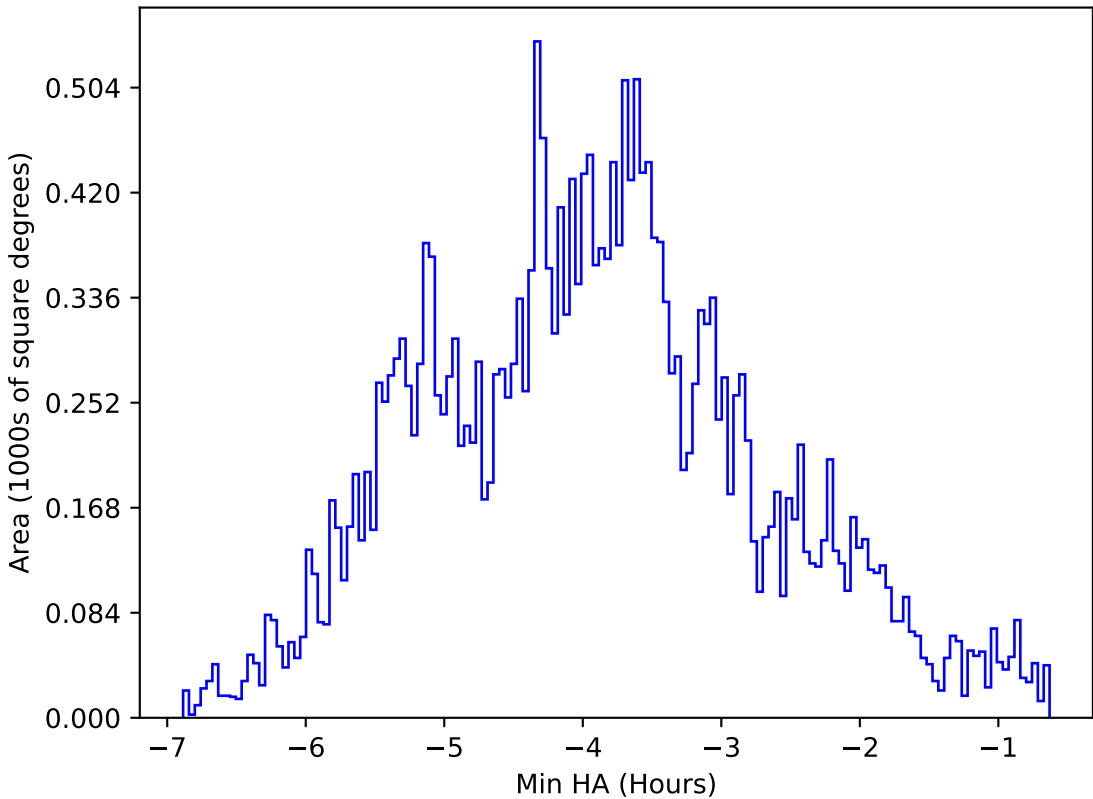
too_elab_heavy_r128_d3_gz_v3.4_10yrs All sky z band: Min HA
