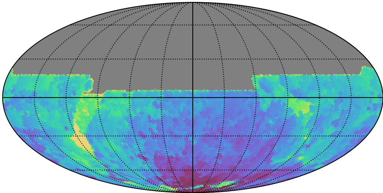
too_elab_heavy_r128_d3_gz_v3.4_10yrs All sky y band: Min HA
