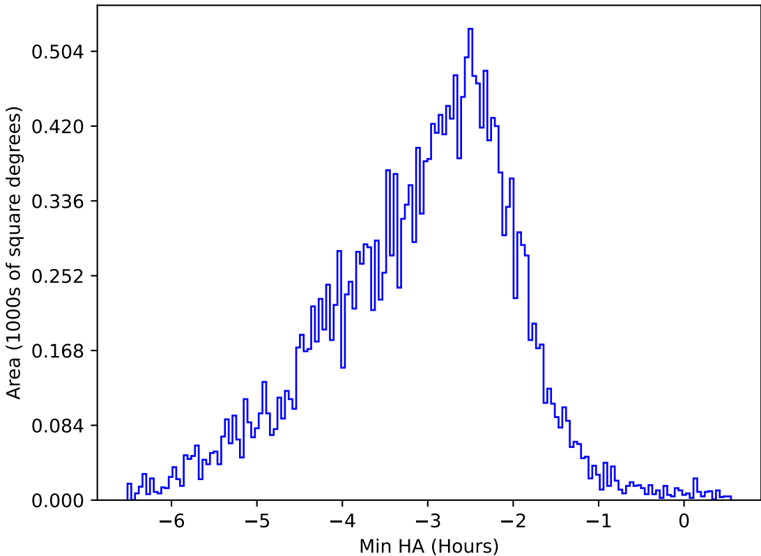
too_elab_heavy_r128_d3_gz_v3.4_10yrs All sky u band: Min HA
