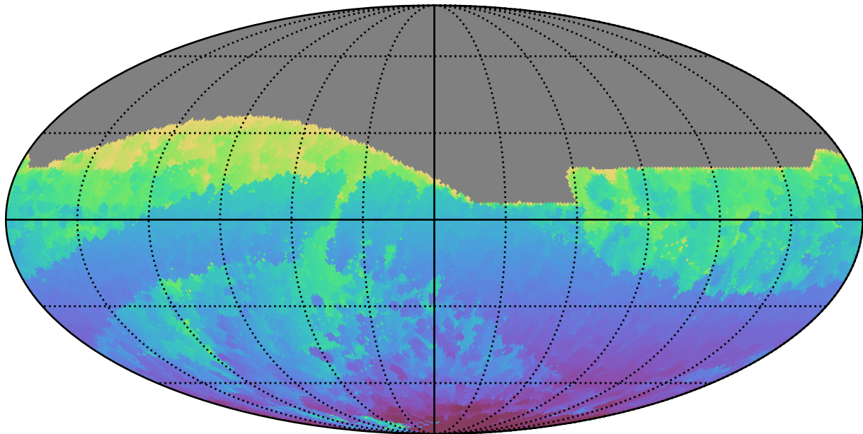
too_elab_heavy_r128_d3_gz_v3.4_10yrs All sky r band: Min HA
