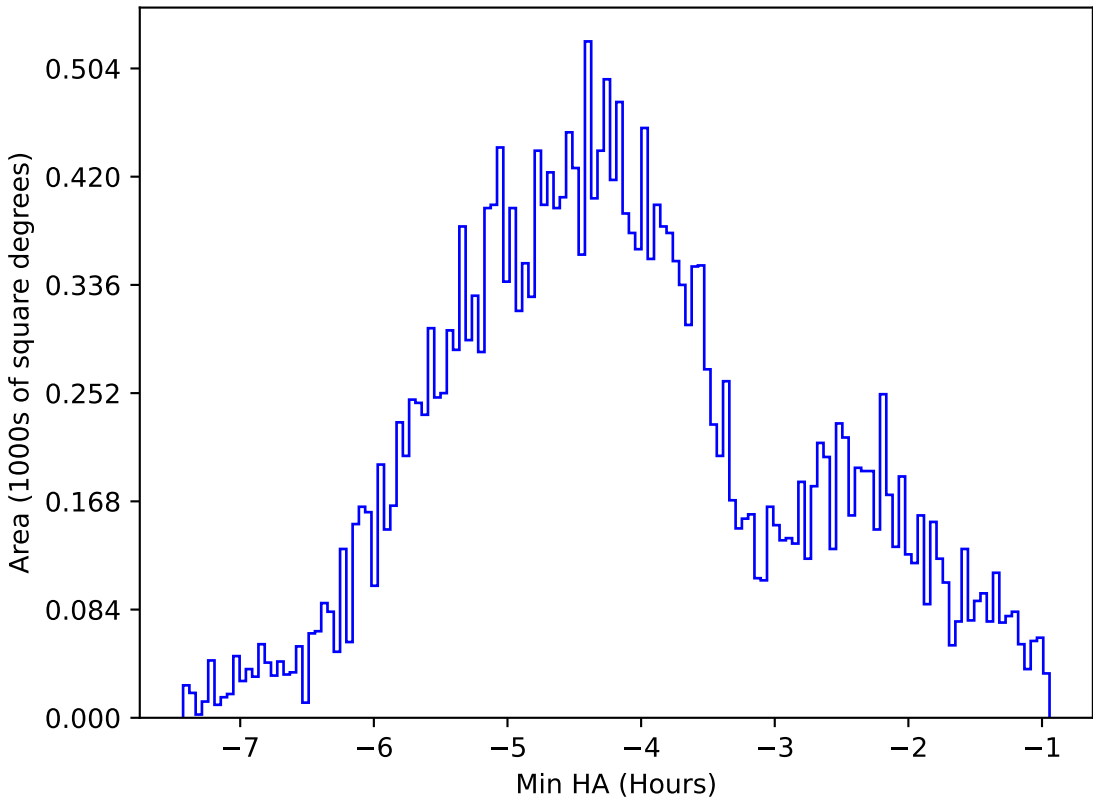
too_elab_heavy_r128_d3_gz_v3.4_10yrs All sky i band: Min HA
