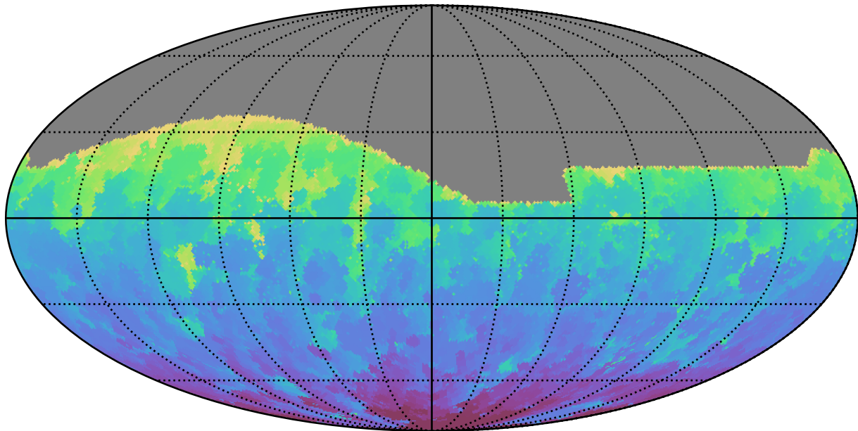
too_elab_heavy_r128_d3_gz_v3.4_10yrs All sky g band: Min HA
