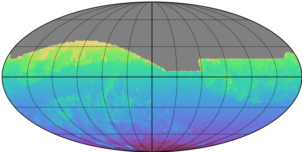
too_elab_heavy_r128_d3_gz_v3.4_10yrs All sky all bands: Min HA
