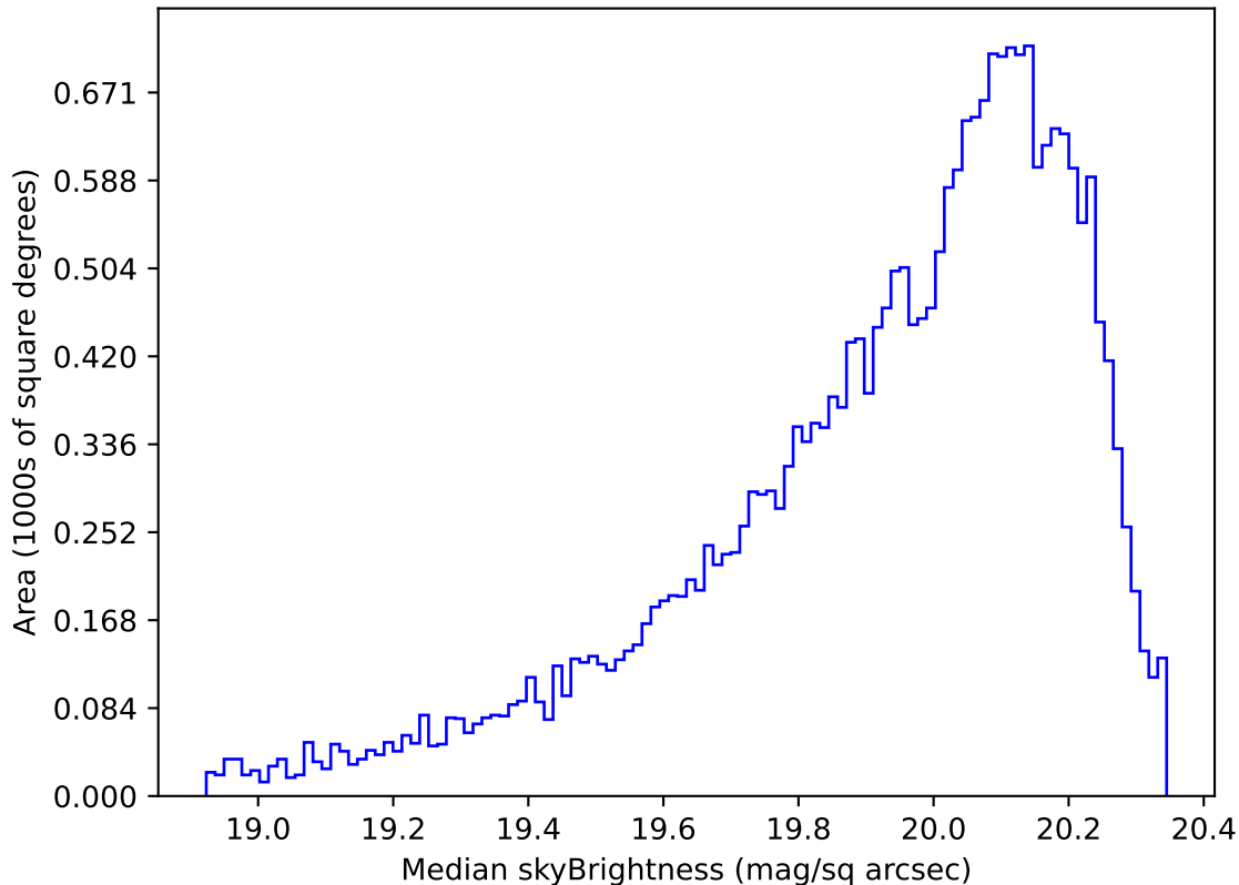
too_elab_heavy_r128_d3_gz_v3.4_10yrs Yr 1 i band: Median skyBrightness
