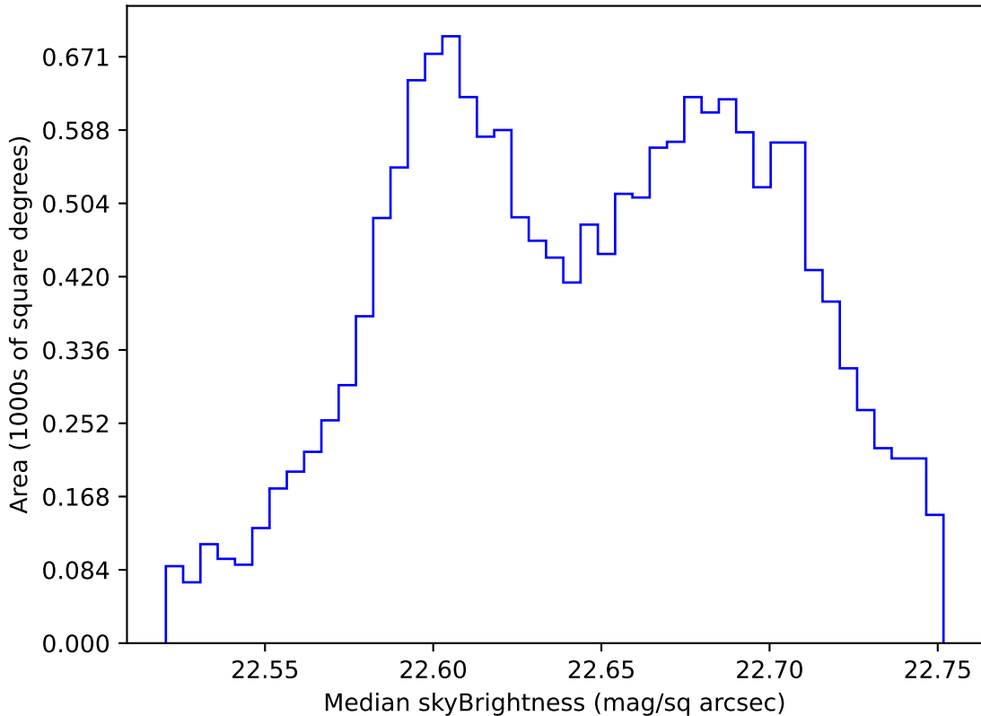
too_elab_heavy_r128_d3_gz_v3.4_10yrs WFD u band: Median skyBrightness
