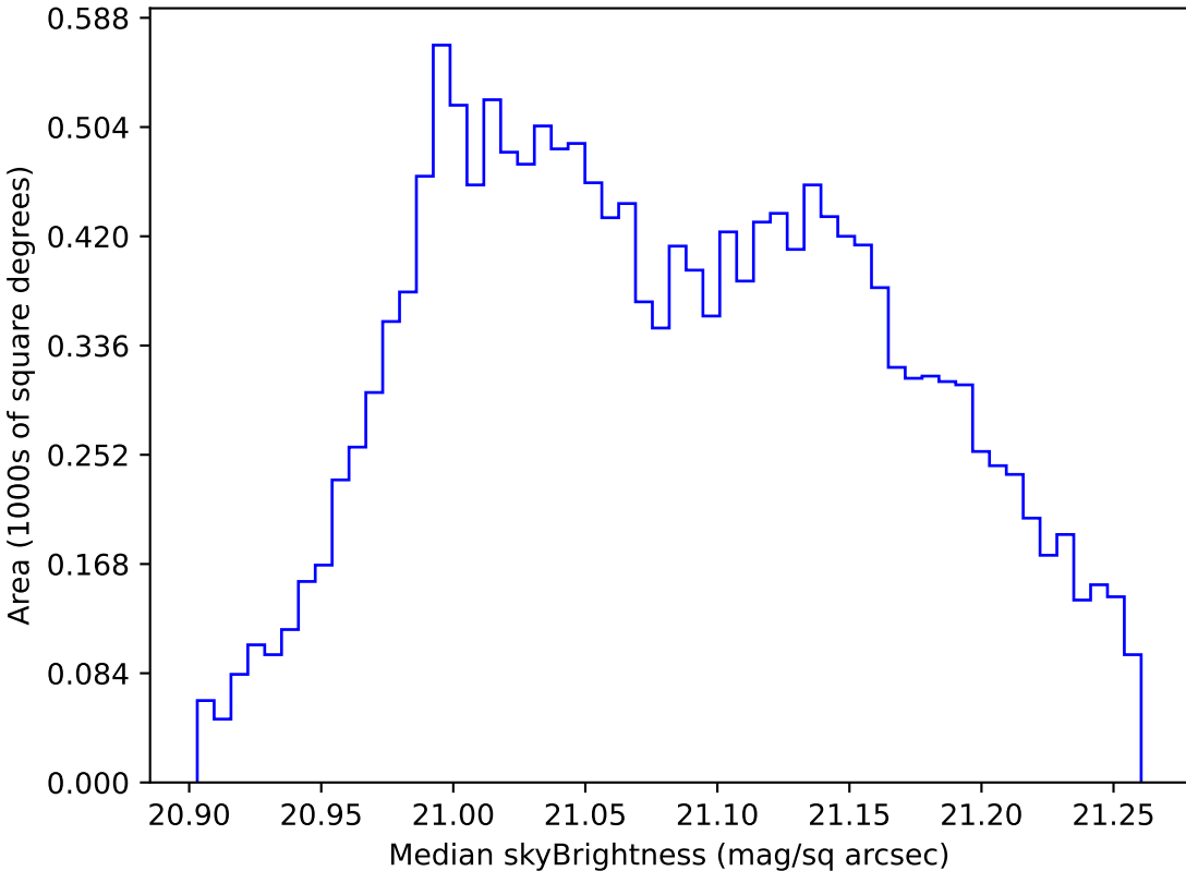
too_elab_heavy_r128_d3_gz_v3.4_10yrs WFD r band: Median skyBrightness
