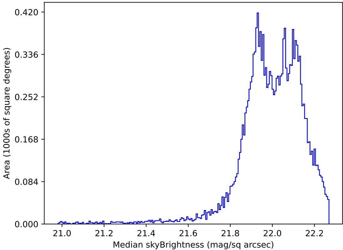
too_elab_heavy_r128_d3_gz_v3.4_10yrs WFD g band: Median skyBrightness
